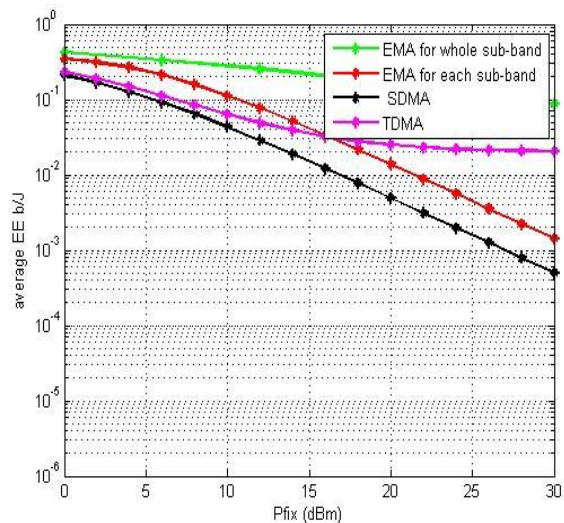
Figure 2: Comparison of the average EE of different MA methods for M=T=30 , N=40 and U=700 .
