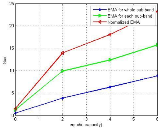
Figure 3: Comparison of gains of different MA methods for M = T = 30 , N = 40 , and U = 700 .
