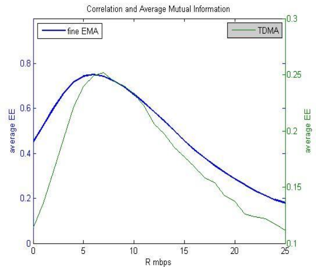
Figure 1: Comparison of the average EE of different MA methods for M=T=2 , N=4 , U=12 , and P_{fix}=45 dBm
