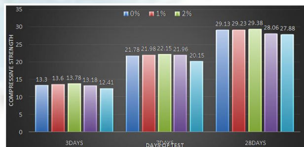
Graph no.1: Compressive strength after 28 days
