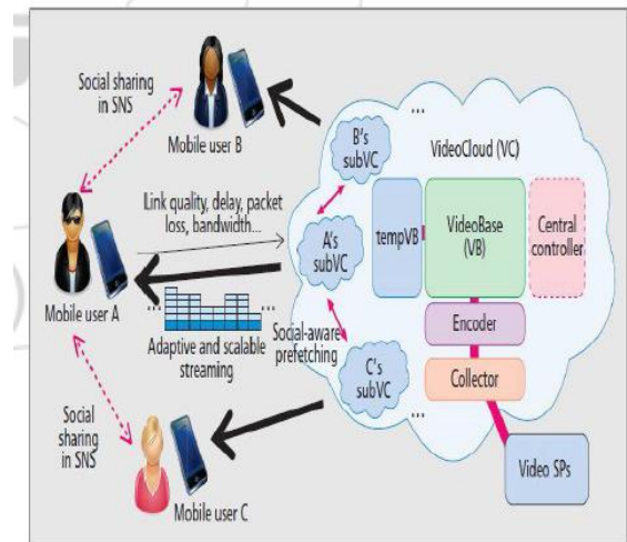
Figure 1: Cloud Frame work
