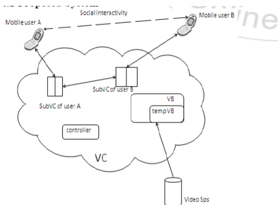
Figure 2: The architecture of the adaptive and efficient way of enhancing the video streaming and sharing of video to the mobile users.
