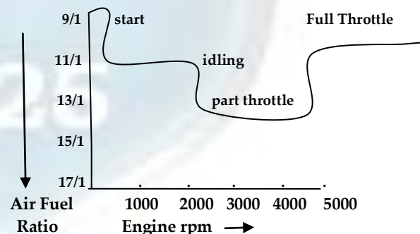
Fig: 3(a) Graph/- Air Fuel Ratio/Engine rpm
